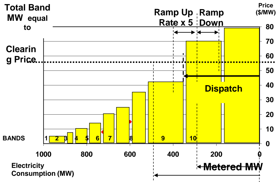
FIGURE 1 : TYPICAL DISPATCH BID FOR SCHEDULED LOAD
