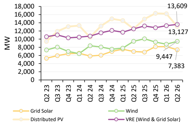
Figure 63 Record highs for combined VRE generation
