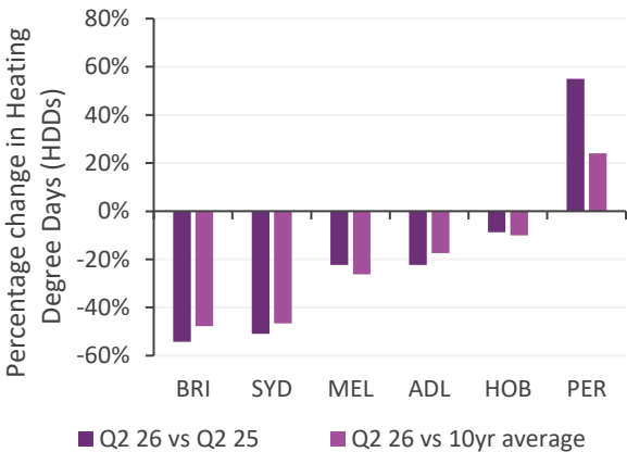
Figure 2 Lower heating requirements across most capital cities in east coast, higher in Perth
