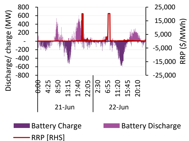
Figure 20 Limited battery charging activity in most South Australian batteries overnight
