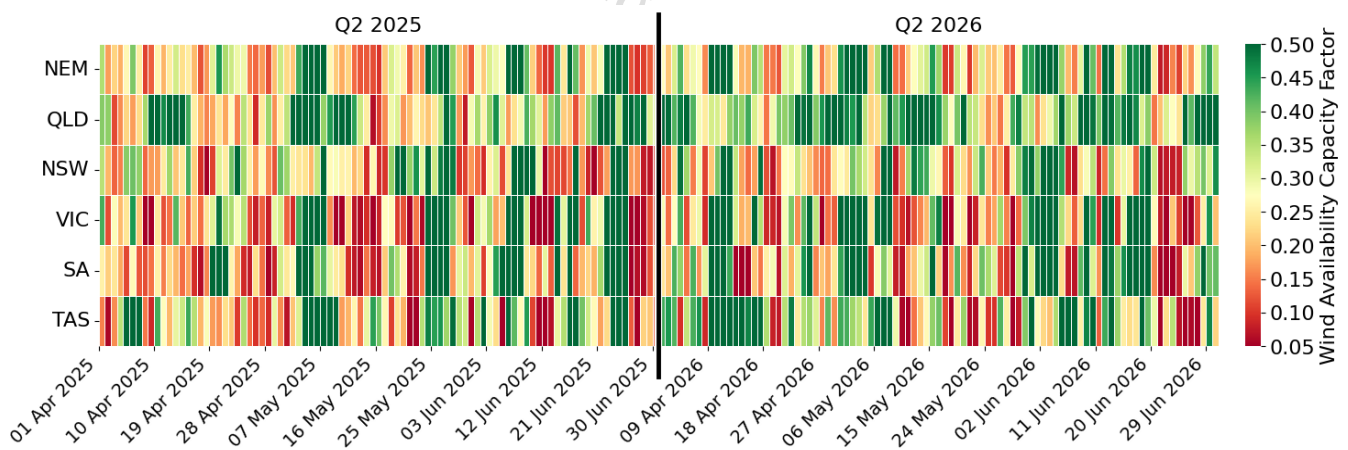
Figure 50 Fewer lows in wind availability across Q2 2026
