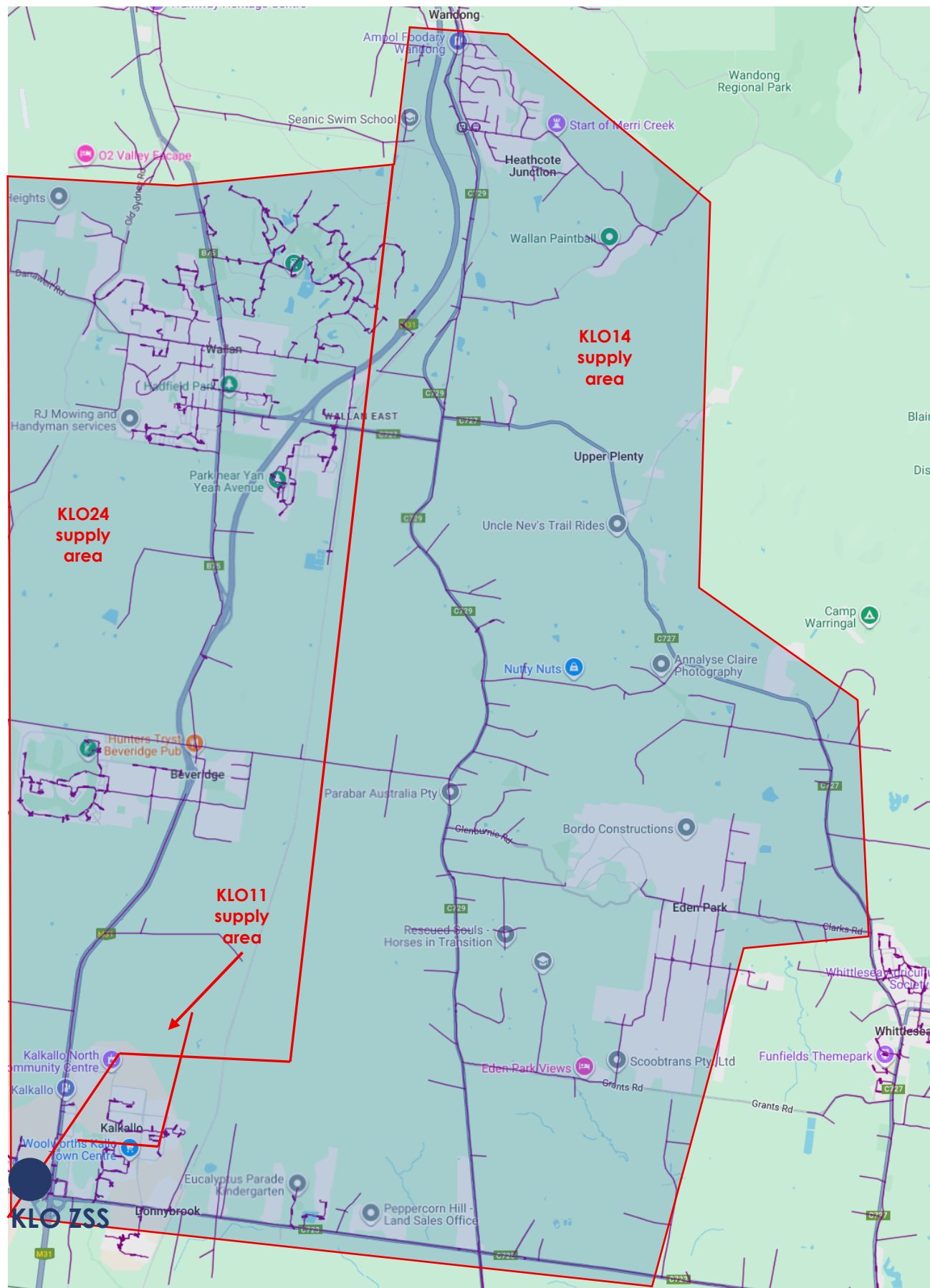
Figure 2: KLO 22 kV network supplying Beveridge, Wallan, parts of Wandong and Whittlesea, and surrounds
