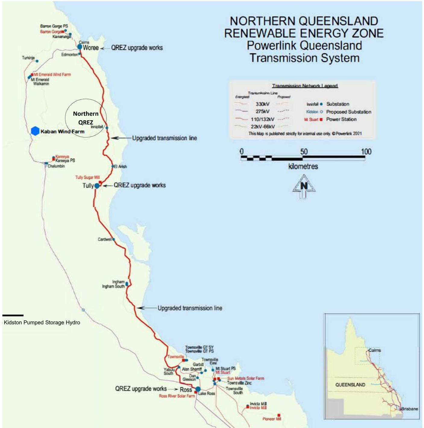
Figure 2: Proposed Northern Queensland Renewable Energy Zone
