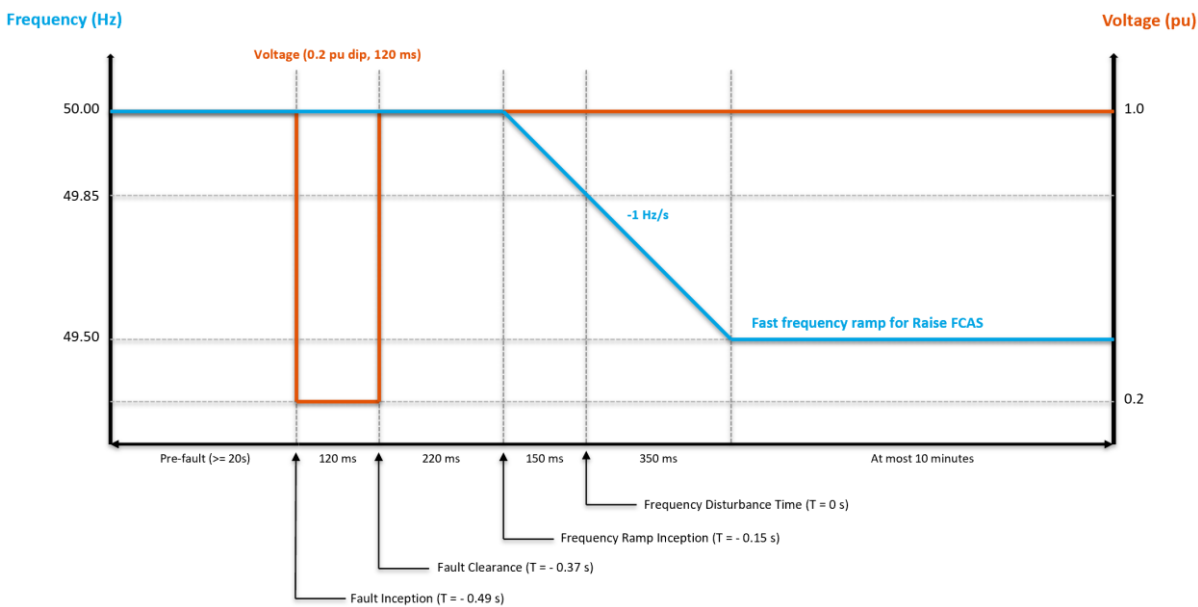
Figure 7 Frequency Ramp with Preceding Voltage Disturbance
