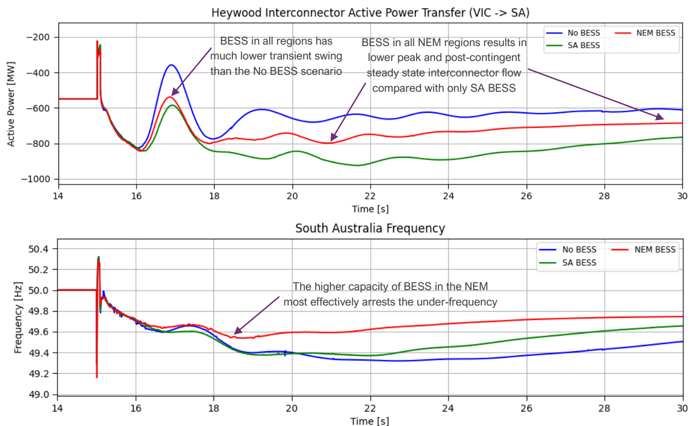
Figure 5 BESS localised to South Australia resulted in the highest post-contingent interconnector flows
