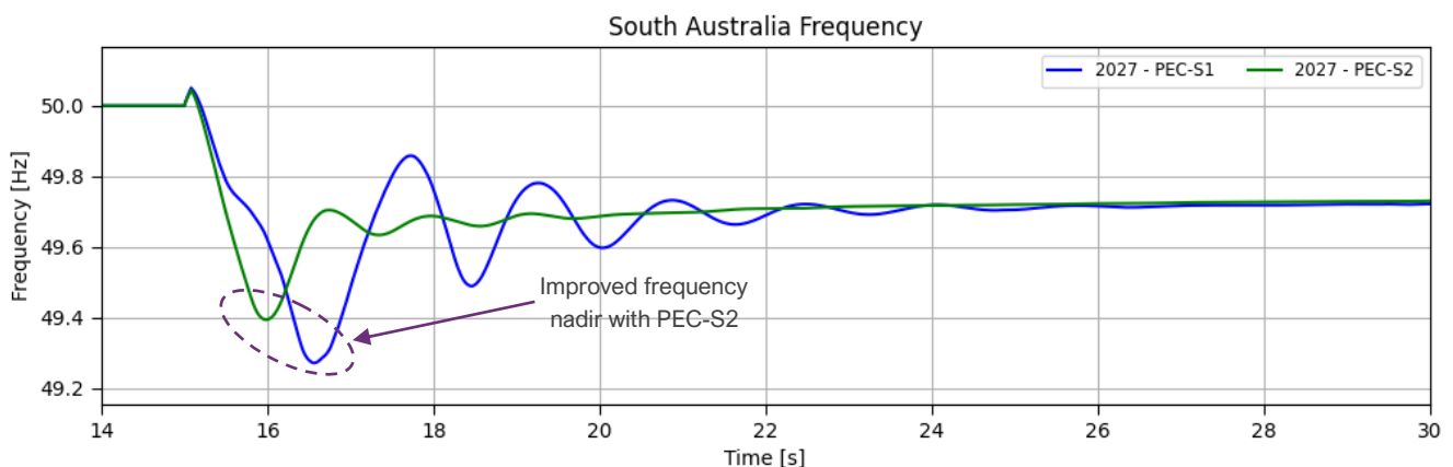
Figure 9 PEC-S2 improves South Australia's frequency response to NEM events
