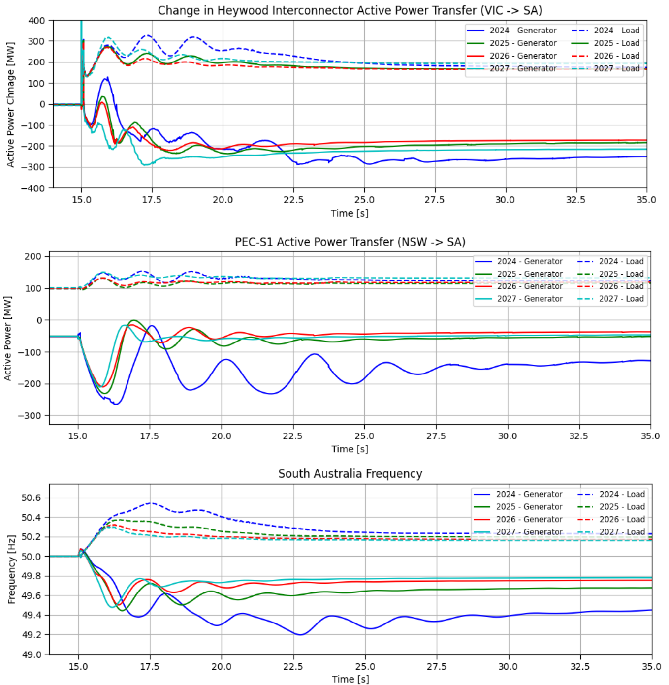
Figure 11 Comparing load and generator contingencies on Heywood Interconnector stability
