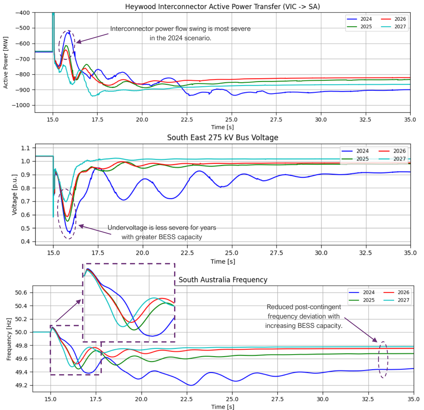
Figure 7 Improving Heywood Interconnector stability with increasing NEM BESS capacity from 2024 to 2027
