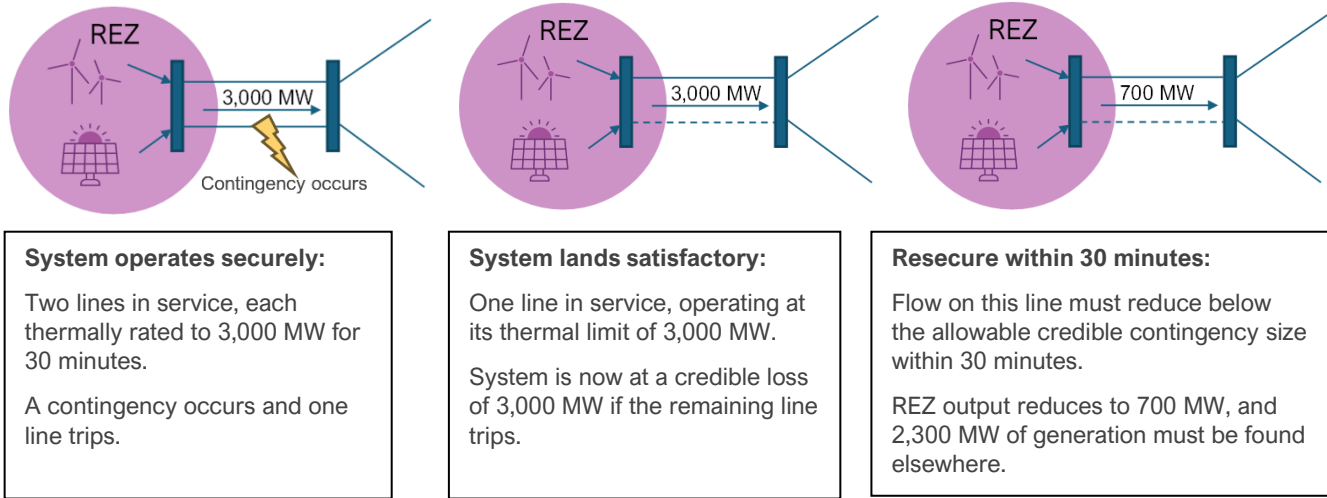
Figure 3 Hypothetical contingency scenario
