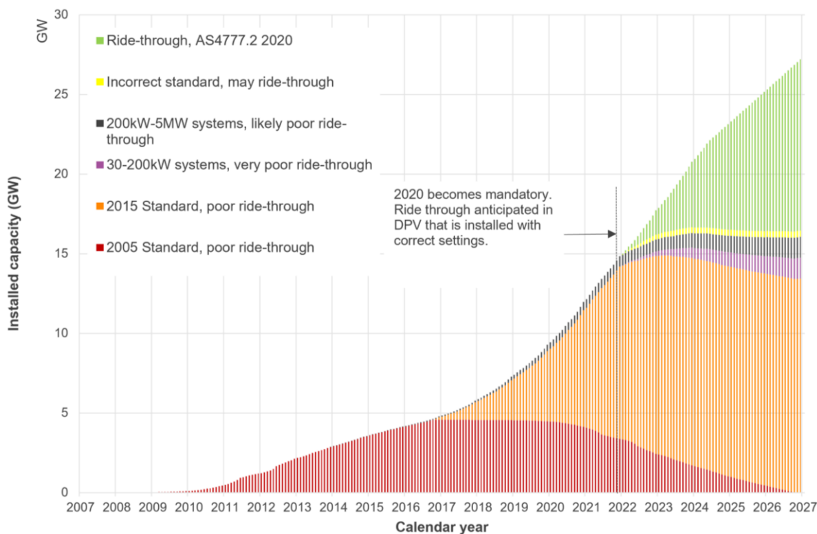
Figure 2 Ride-through capabilities of the installed distributed PV fleet in the NEM
