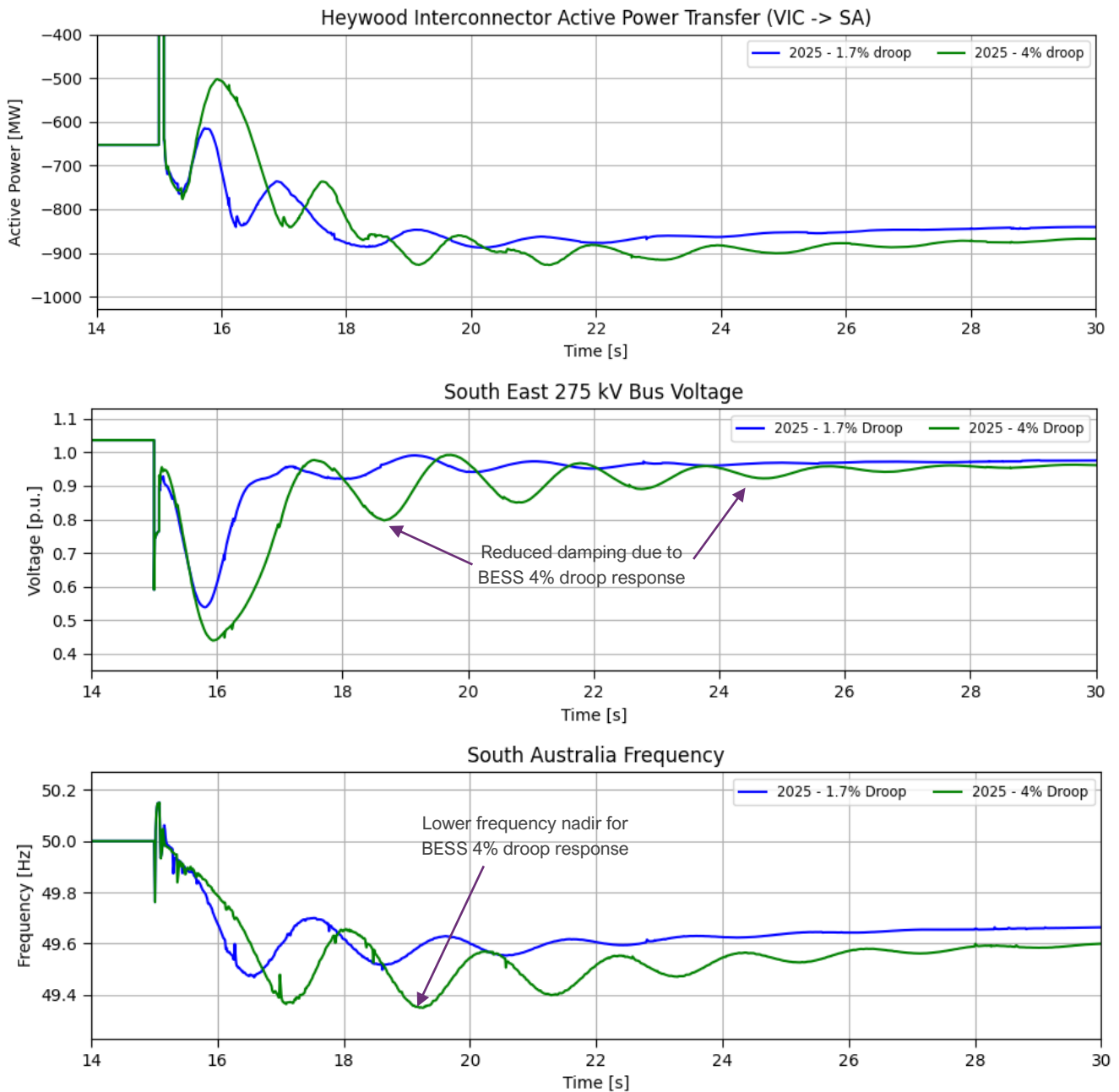
Figure 10 1.7% BESS frequency droop settings offer benefits compared to 4% frequency droop
