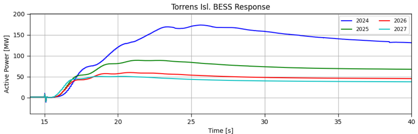
Figure 6 Reducing individual BESS contribution from 2024 to 2027
