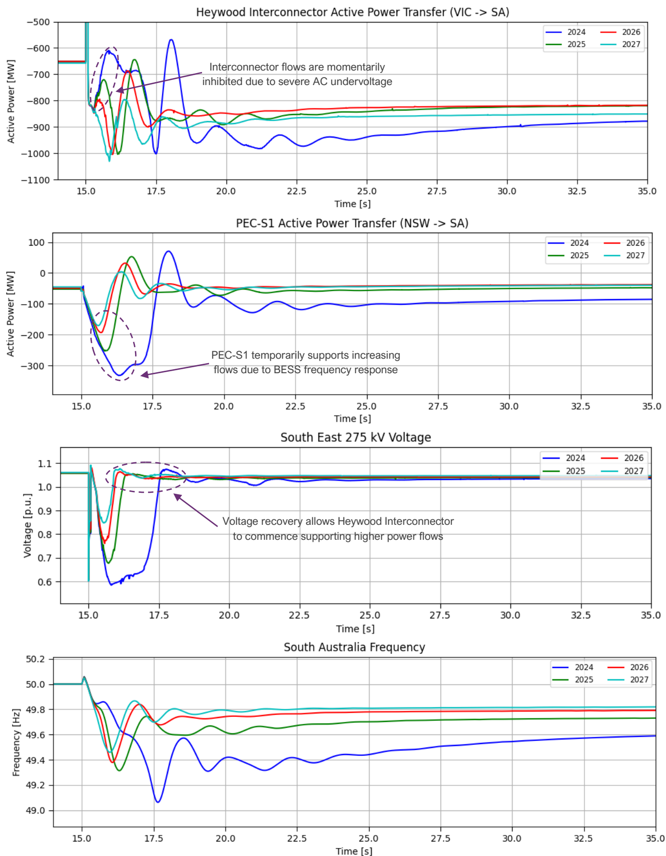
Figure 8 PEC-S1 supports Heywood Interconnector stability during the transient period
