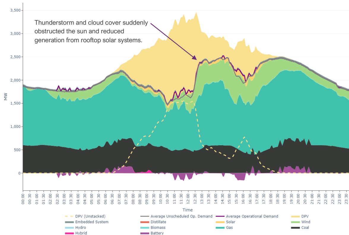
Figure 1 Rapid upswing in electricity demand in Western Australia's SWIS on 13 March 2025
