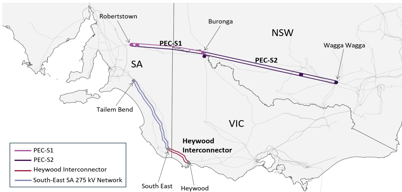
Figure 4 Transmission network overview showing Heywood and PEC interconnectors
