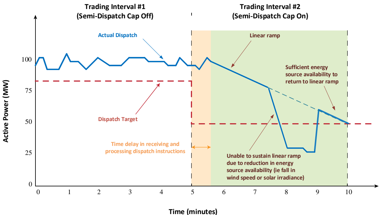
Figure 3 Figure 7 Semi-scheduled generating unit cannot sustain linear ramp due to reduction in energy available
