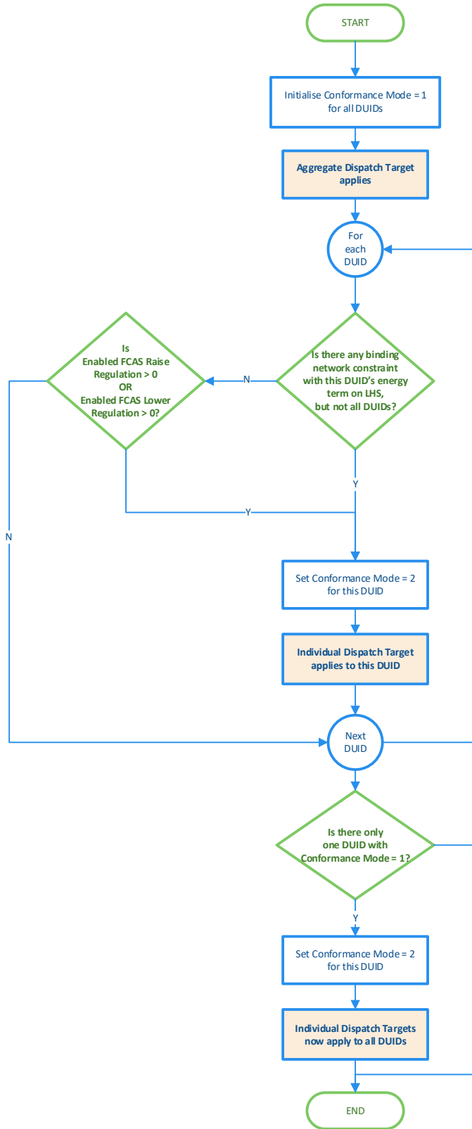
Figure 2 Dispatch conformance logic for a Mixed Aggregate
