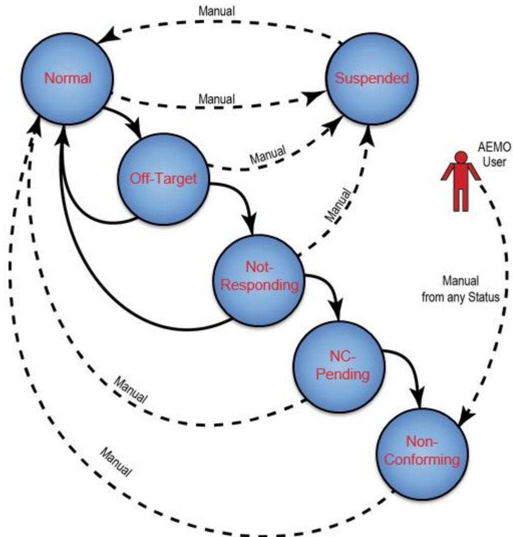
Figure 5 Figure 9 Status Transition in Auto Mode
