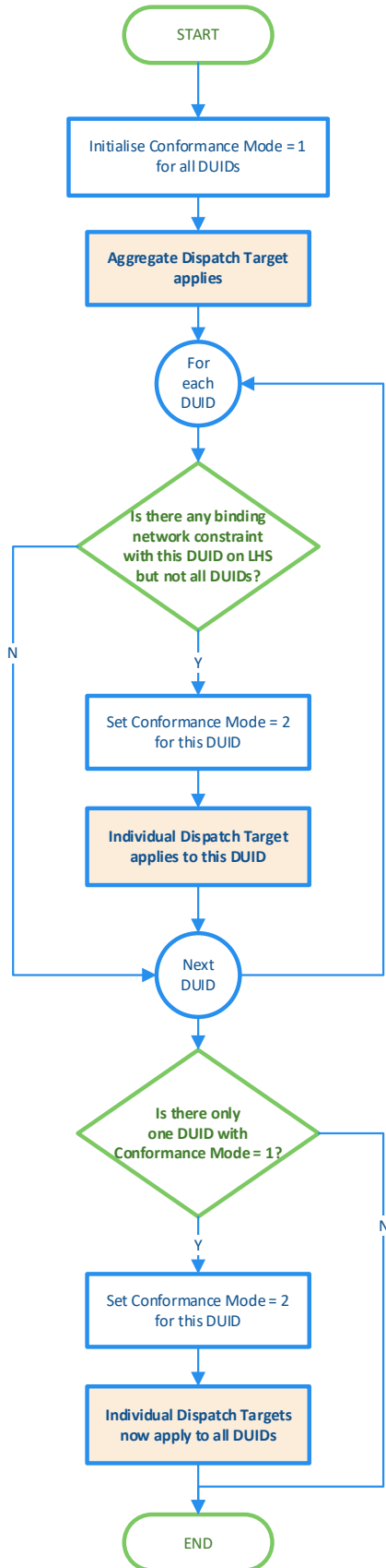
Figure 2 Dispatch conformance logic for a Target Aggregate
