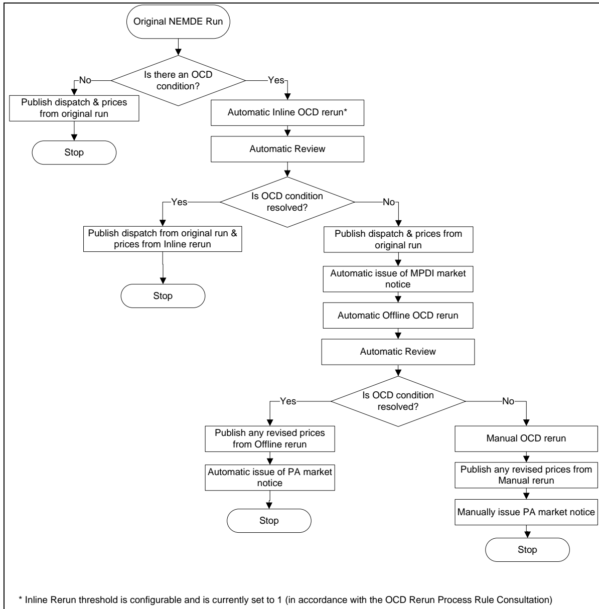
Figure 3 Figure 7 Over Constrained Dispatch Re-run Flow Diagram
