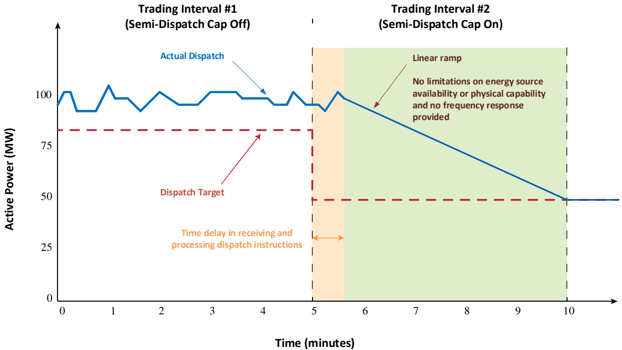
Figure 1 Figure 5 Semi-scheduled generating unit linear ramping with no limiting factors
