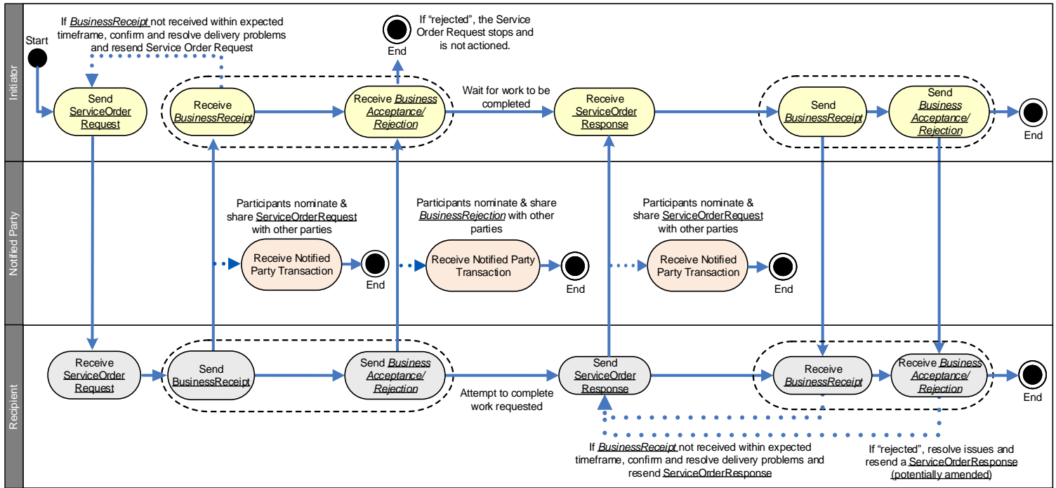
Figure 1 Service Orders
