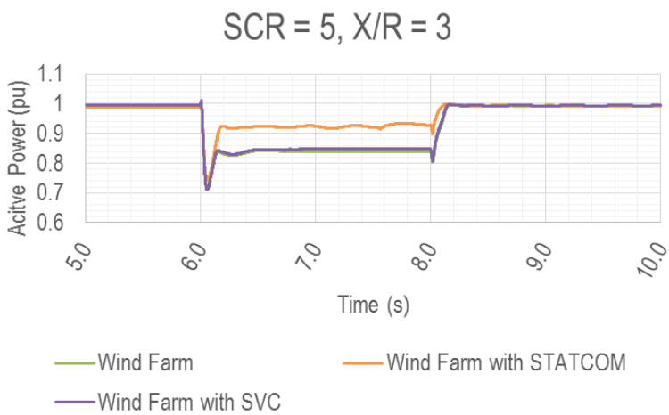
Figure 35 Active power
