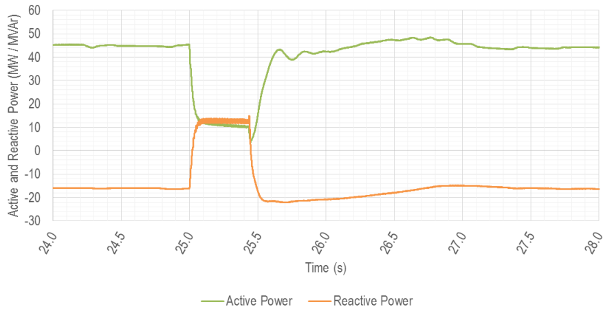
Figure 19 Solar Farm B POC active and reactive power
