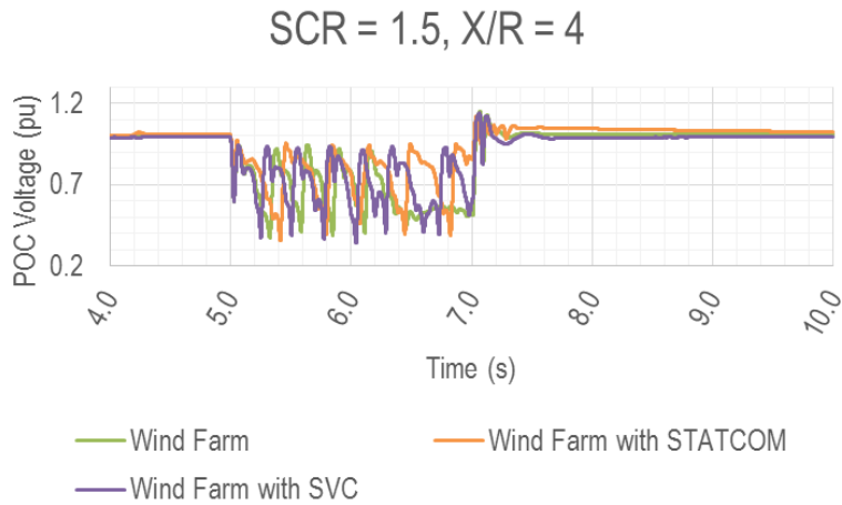
Figure 42 Voltage at point of connection
