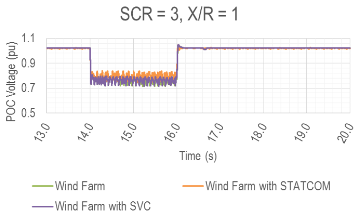
Figure 34 Voltage at point of connection
