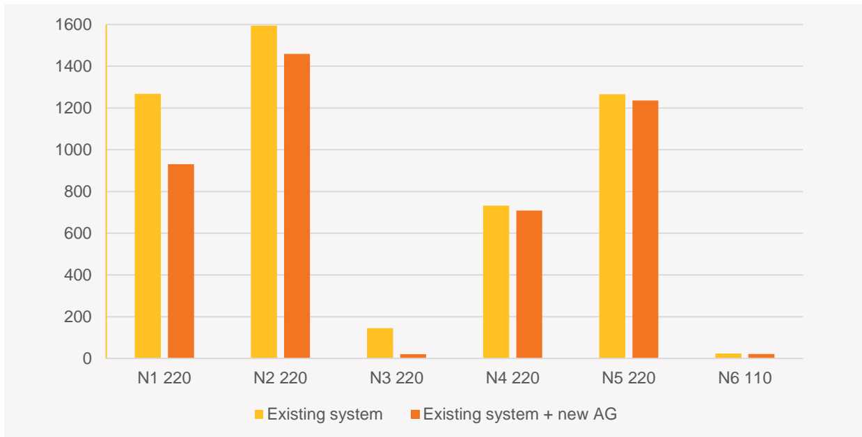
Figure 5 Assessment of available fault level at six Tasmanian busbar locations (new AG at N1 220)
