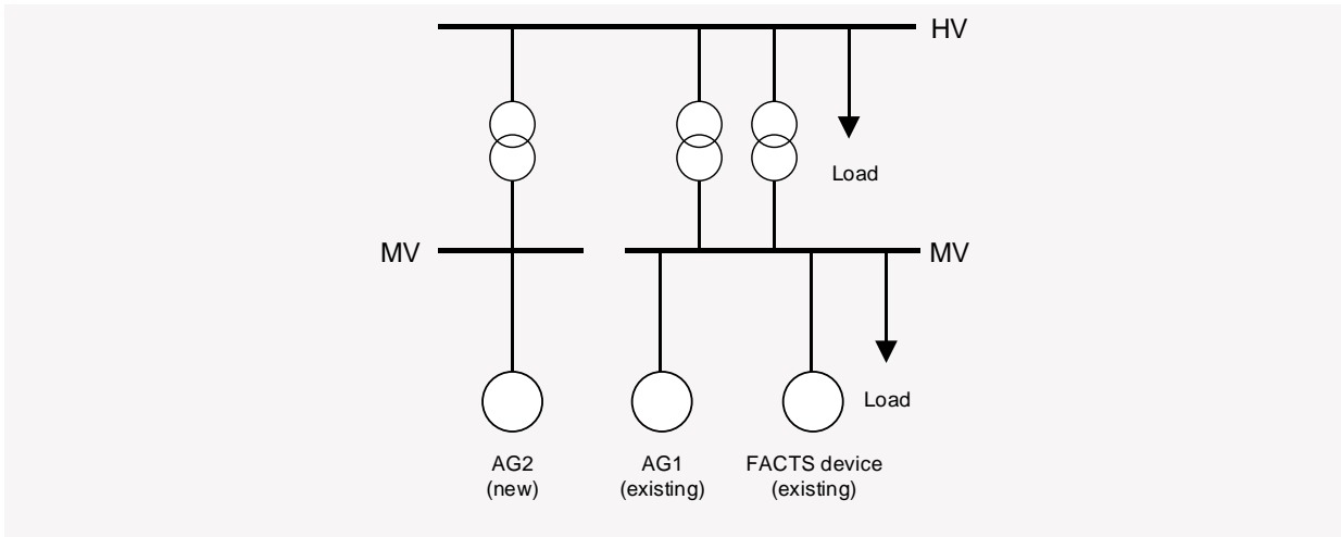
Figure 6 Single line diagram of substation under study
