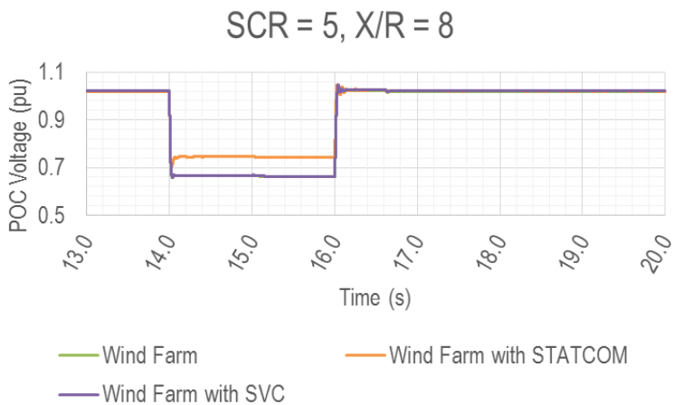
Figure 38 Voltage at point of connection
