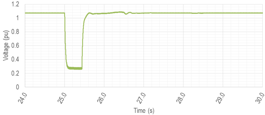
Figure 16 Solar Farm A POC voltage
