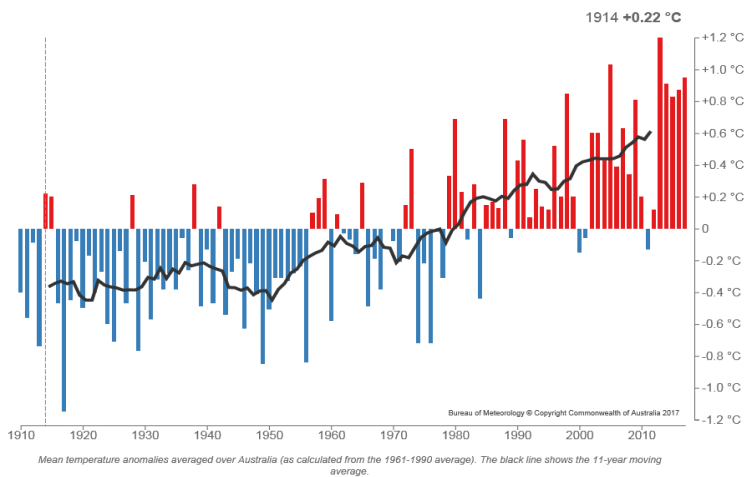
Figure 20 Australian mean temperature anomaly
