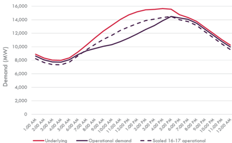
Figure 24 Changing load shape is resulting in a shorter and later operational demand peak
