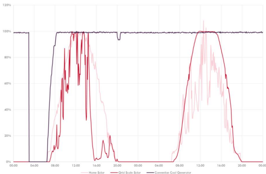
Figure 26 Residual uncertainty of conventional and solar generation
