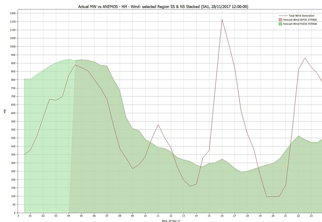
Figure 27 Day-ahead forecast compared with actual wind output in South Australia, 29 November 2017 (case study 1)
