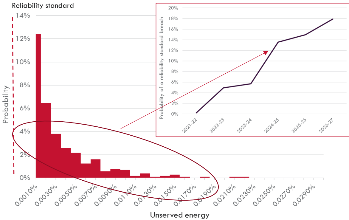
Figure 44 Distribution of annual USE showing probability that reliability standard will be breached, 2024-25
