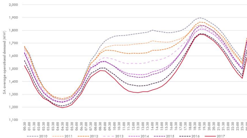
Figure 16 Effect of growing rooftop solar
