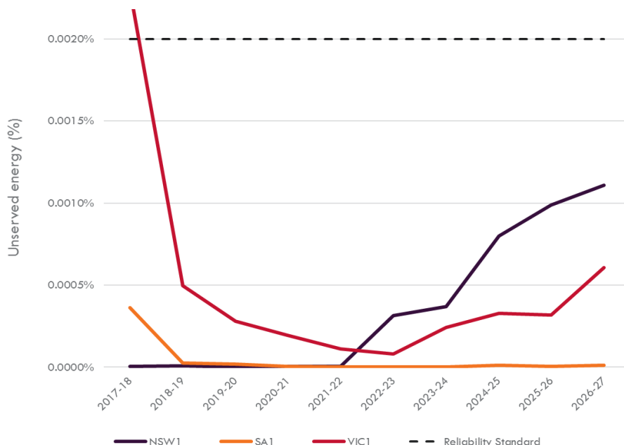
Figure 43 Assessing supply adequacy against the reliability standard
