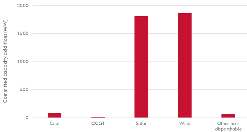
Figure 14 Committed changes in generating capacity in the NEM
