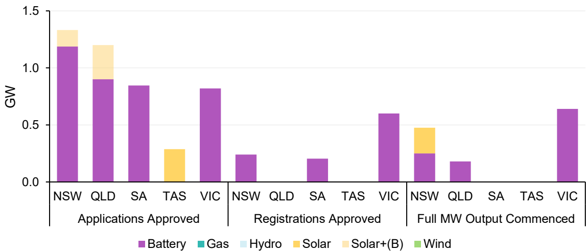
Figure 63 Strong quarter for battery project milestones
