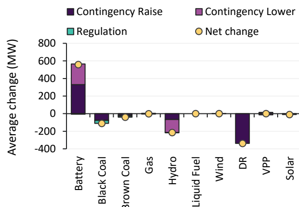
Figure 72 Battery enablement increased across contingency FCAS services
