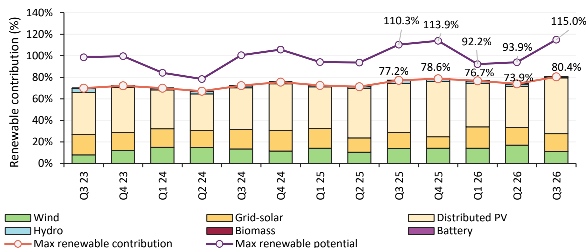
Figure 58 Peak renewable and storage contribution sets a new record
