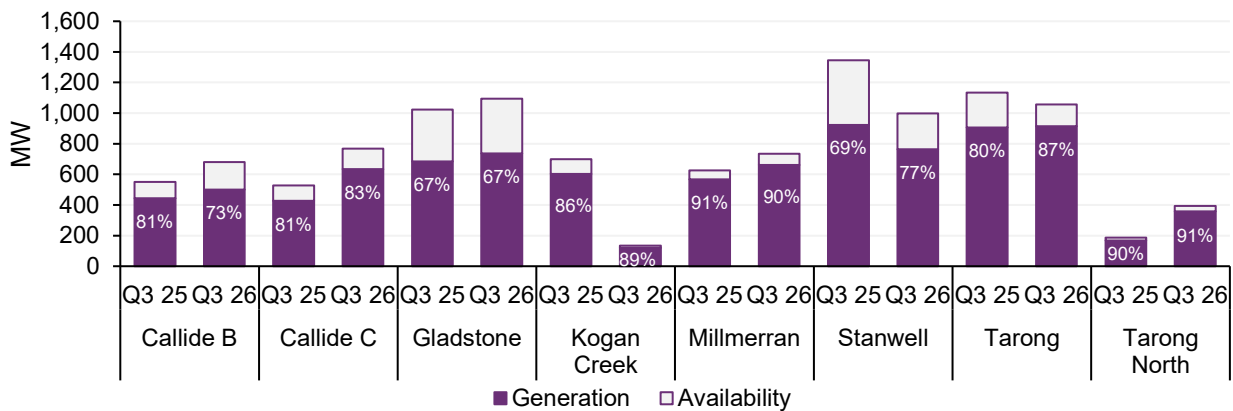
Figure 35 Queensland black coal-fired output decreased year-on-year driven by Kogan Creek and Stanwell
