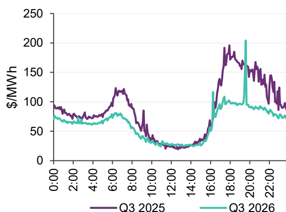
Figure 15 Significant reduction in spot prices during the evening peak, while morning peak and overnight prices also declined
