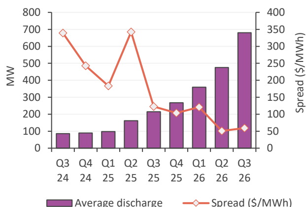
Figure 56 NEM-wide battery price spread
