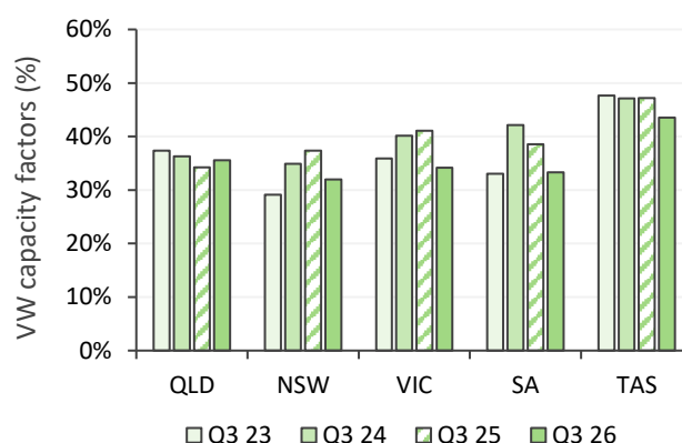
Figure 45 Wind availability down across most regions
