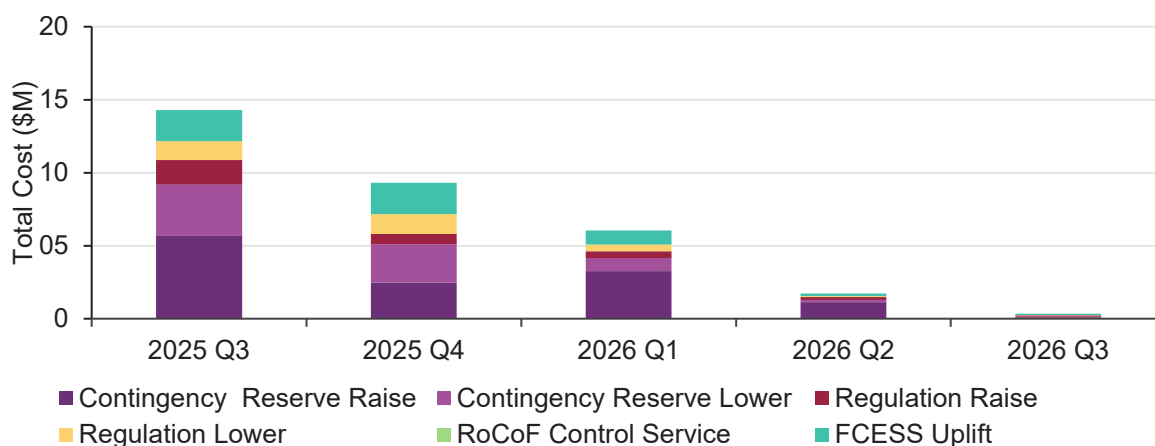
Figure 112 Falling FCESS costs in the WEM
