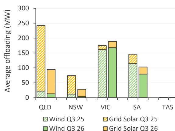
Figure 49 Queensland experienced the largest reduction in offloading
