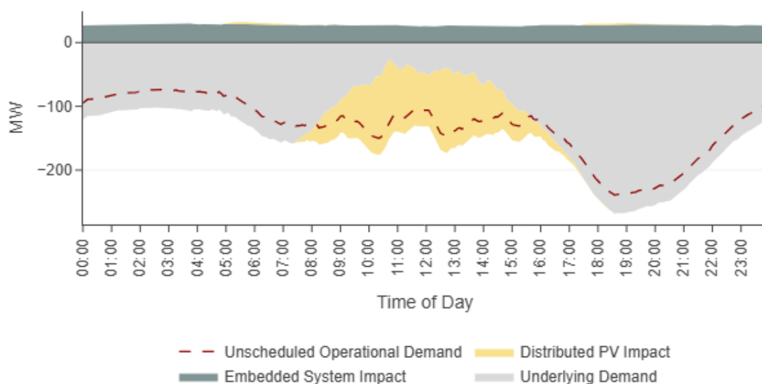
Figure 98 Decreased unscheduled operational demand at all times of day
