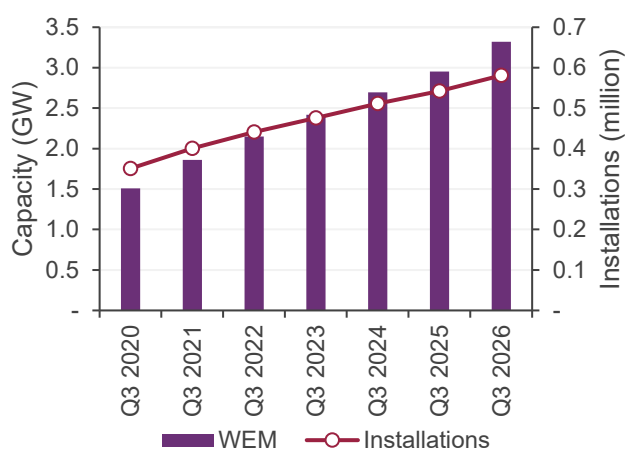
Figure 99 Steady growth in rooftop solar capacity and installations in the WEM
