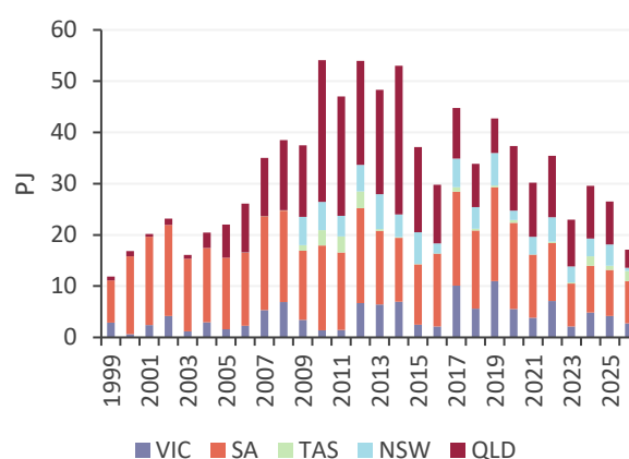
Figure 85 Lowest Q3 demand for gas-fired generation since 2003
