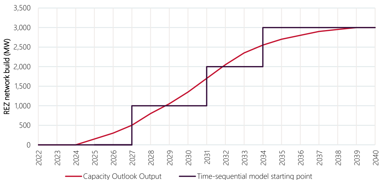
Figure 25 Figure 14 Conversion of linearised REZ expansion to network upgrade options
