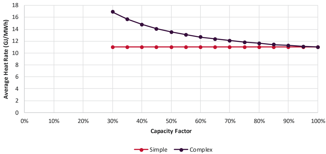
Figure 28 Figure 17 Example of heat rates – simple versus complex
