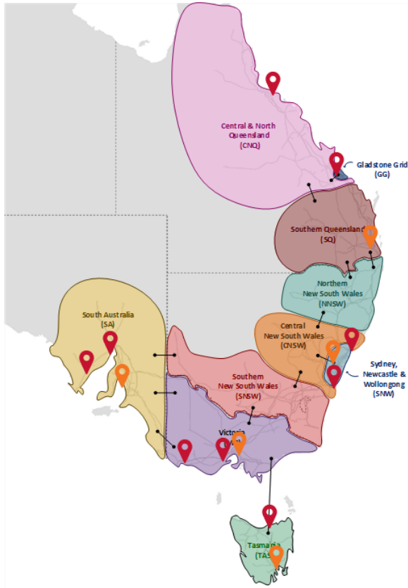
Figure 16 Electrolyser locations and their connections to electricity nodes
