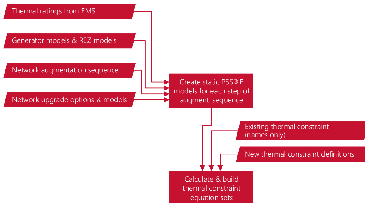
Figure 18 Thermal constraint equation process
