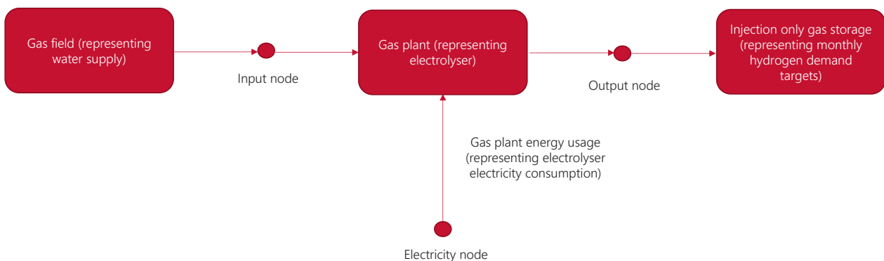
Figure 15 Hydrogen implementation in capacity outlook models
