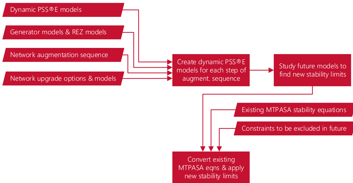
Figure 30 Figure 19 Stability constraint equation process
