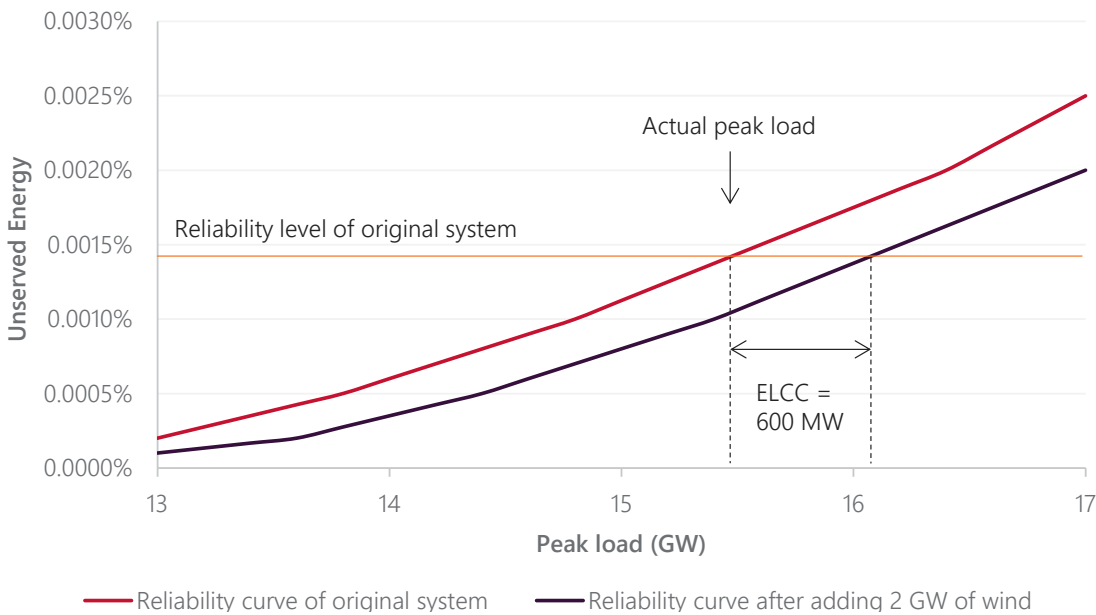
Figure 23 Figure 12 Example calculation of effective load carrying capability
