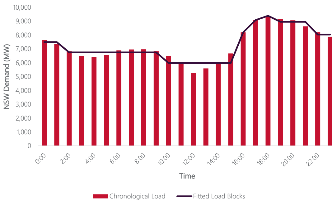
Figure 11 Example representation of fitted load blocks
