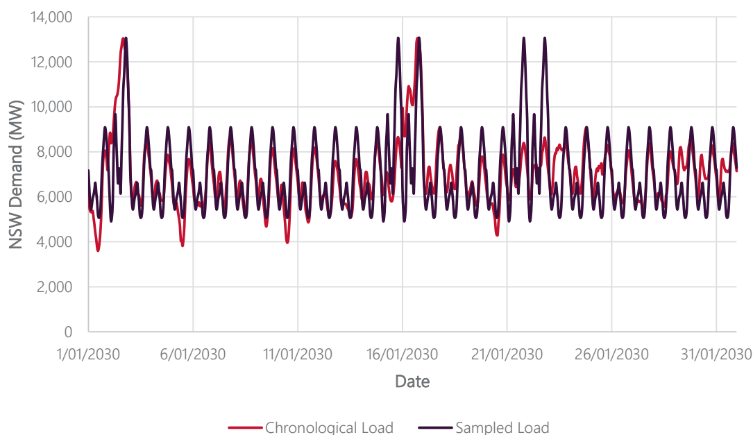
Figure 21 Figure 10 Example representation of a sampled load profile
