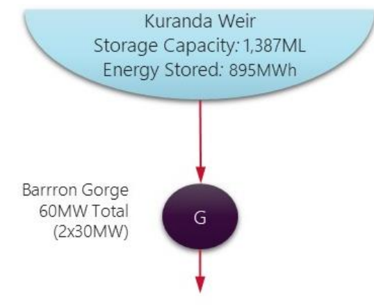
Figure 12— Barron Gorge power station hydro model
