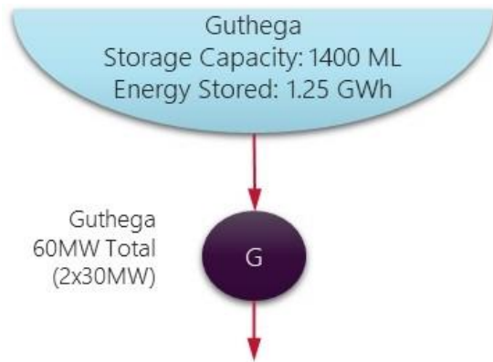
Figure 16—Guthega power station hydro model
