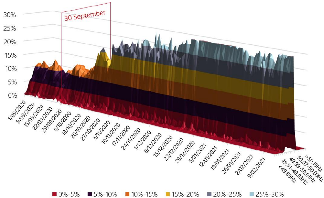
Figure 2 Daily frequency distribution (data from 01 Sep 2020 to 15 Feb 2021)
