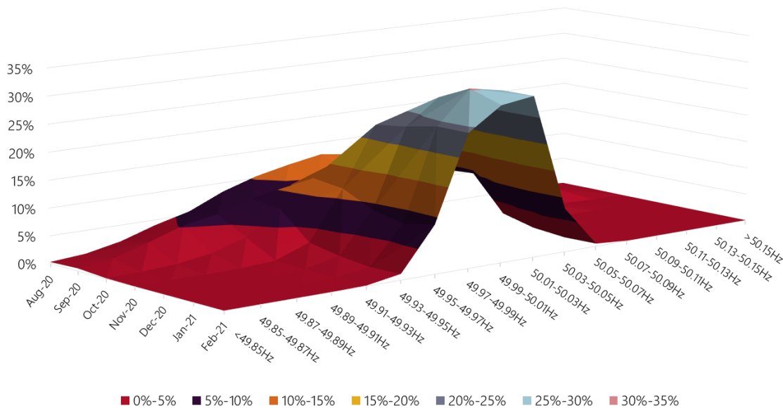
Figure 1 Monthly frequency distribution (six-month rolling, 01 Aug 2020 to 15 Feb 2021)
