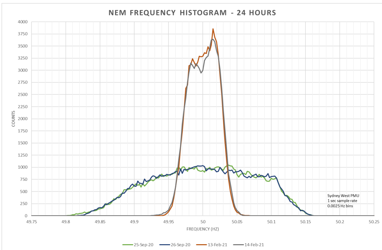
Figure 3 Comparison of NEM frequency distribution – Sep 2020 vs Feb 2021
