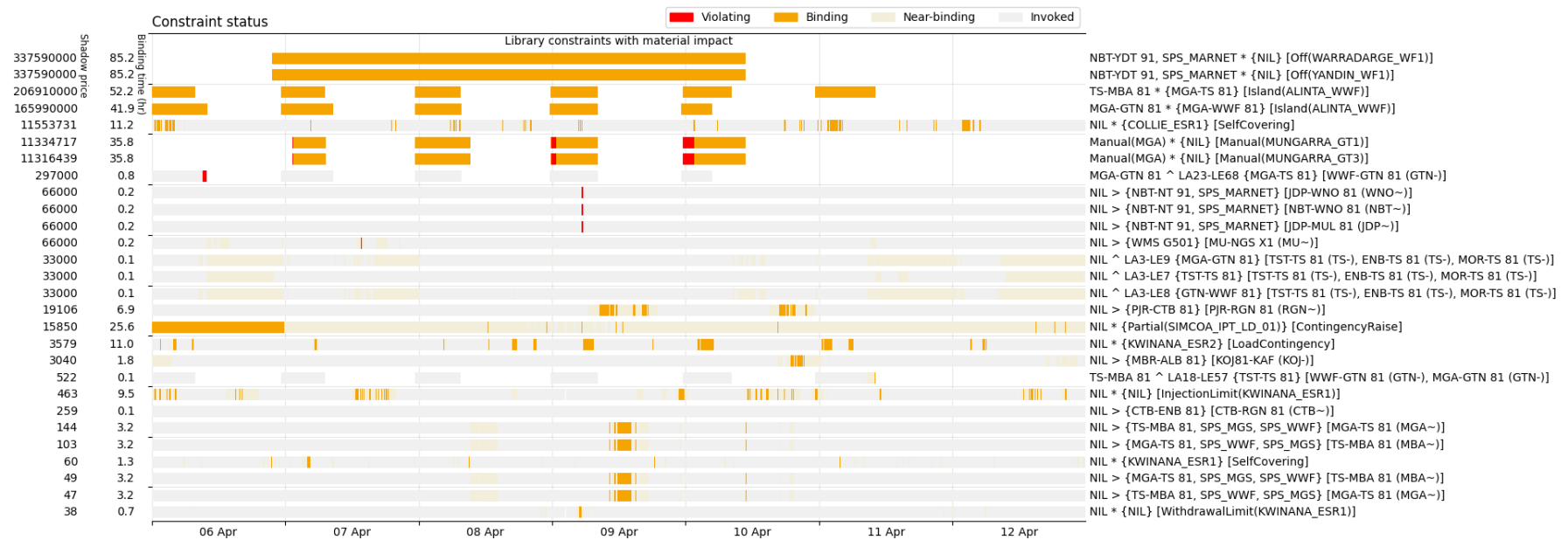
Figure 3 – Binding summary of library constraints.
