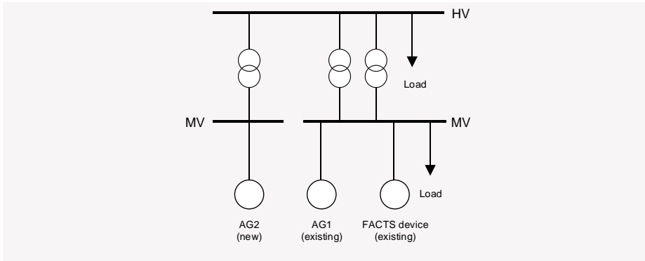
Figure 6 Single line diagram of substation under study
