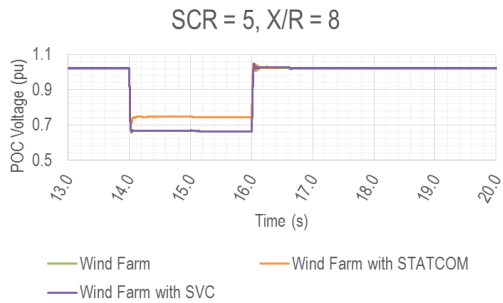
Figure 38 Voltage at point of connection
