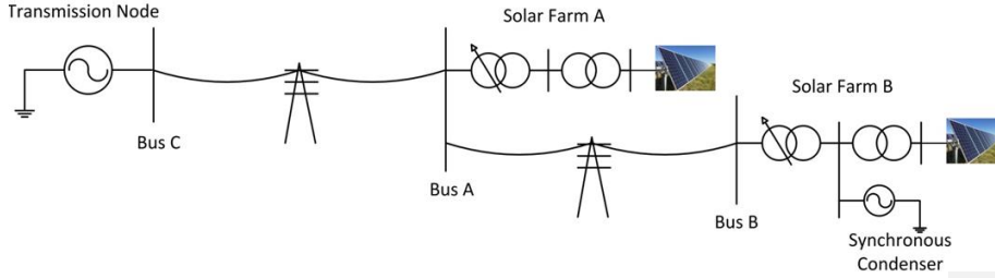
Figure 25 Solar Farm A and B POC voltage
