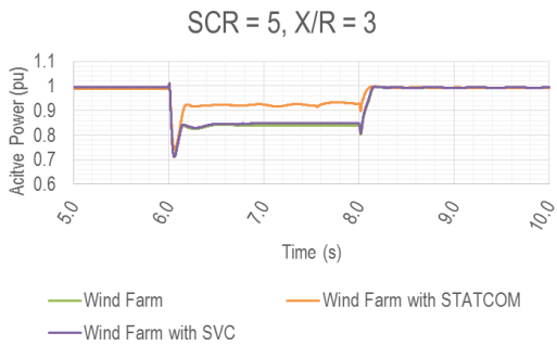
Figure 35 Active power
