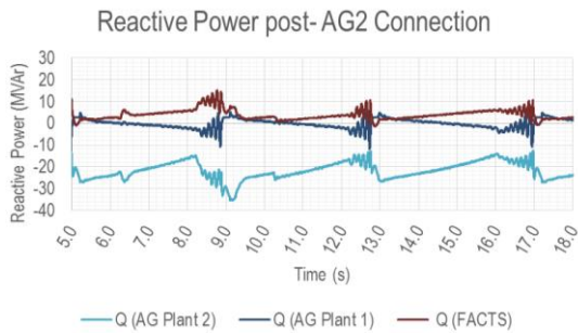
Figure 12 Dynamic behaviour of sub network post-AG2 connection
