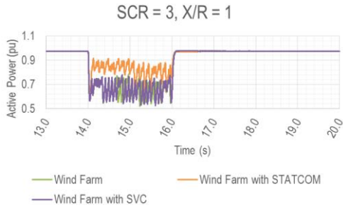
Figure 34 Voltage at point of connection
