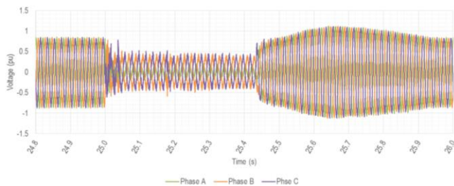
Figure 20 Solar Farm A inverter terminal voltage
