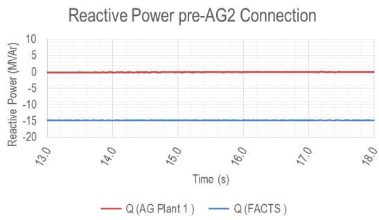
Figure 9 Dynamic behaviour of sub network pre-AG2 connection
