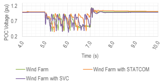
Figure 42 Voltage at point of connection
