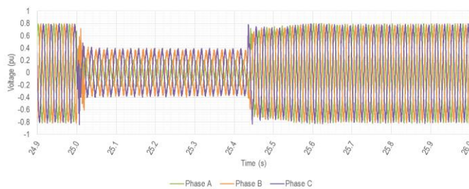
Figure 14 Solar Farm A inverter terminal voltage
