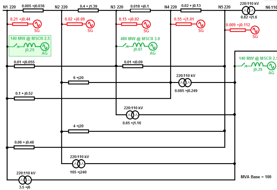
Figure 4 Study on impact of new AG (shaded) on Tasmanian power system
