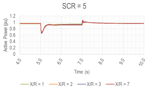
Figure 27 Active power
