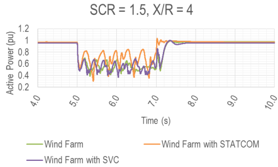
Figure 41 Active power
