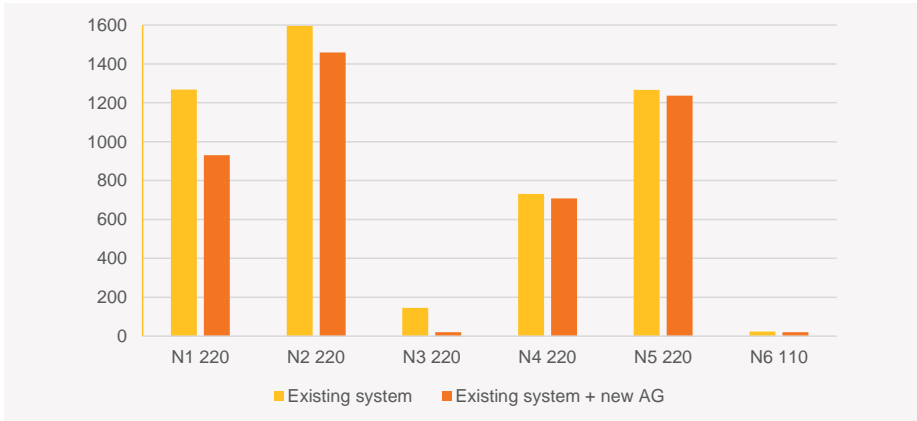
Figure 5 Assessment of available fault level at six Tasmanian busbar locations (new AG at N1 220)
