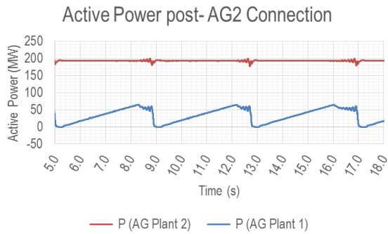
Figure 11 Dynamic behaviour of sub network post-AG2 connection
