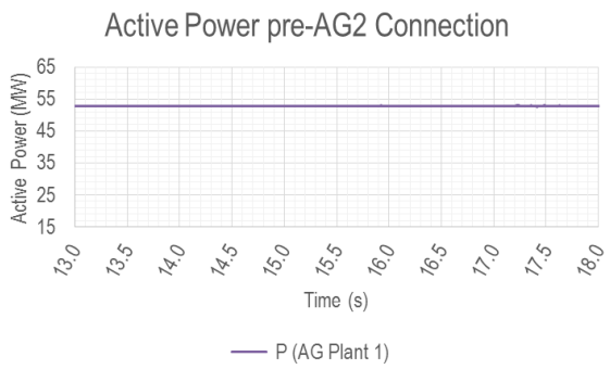
Figure 9 Dynamic behaviour of sub network pre-AG2 connection
