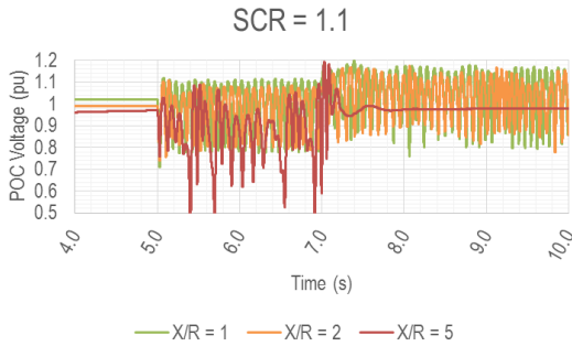
Figure 32 Voltage at point of connection
