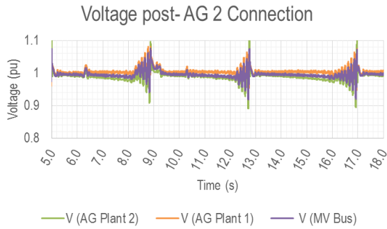
Figure 10 Dynamic behaviour of sub network post-AG2 connection
