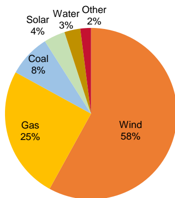
Figure 4: Proposed generation
