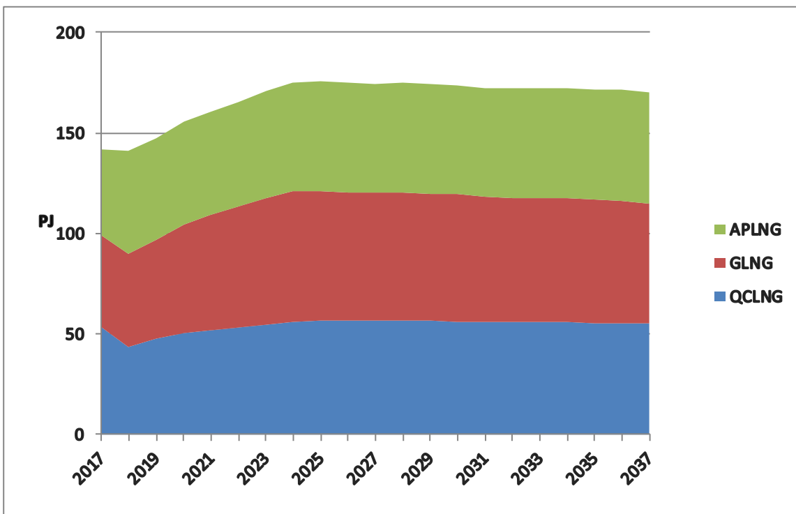
Figure 4-6 Grid electricity usage in compression, Neutral Scenario
