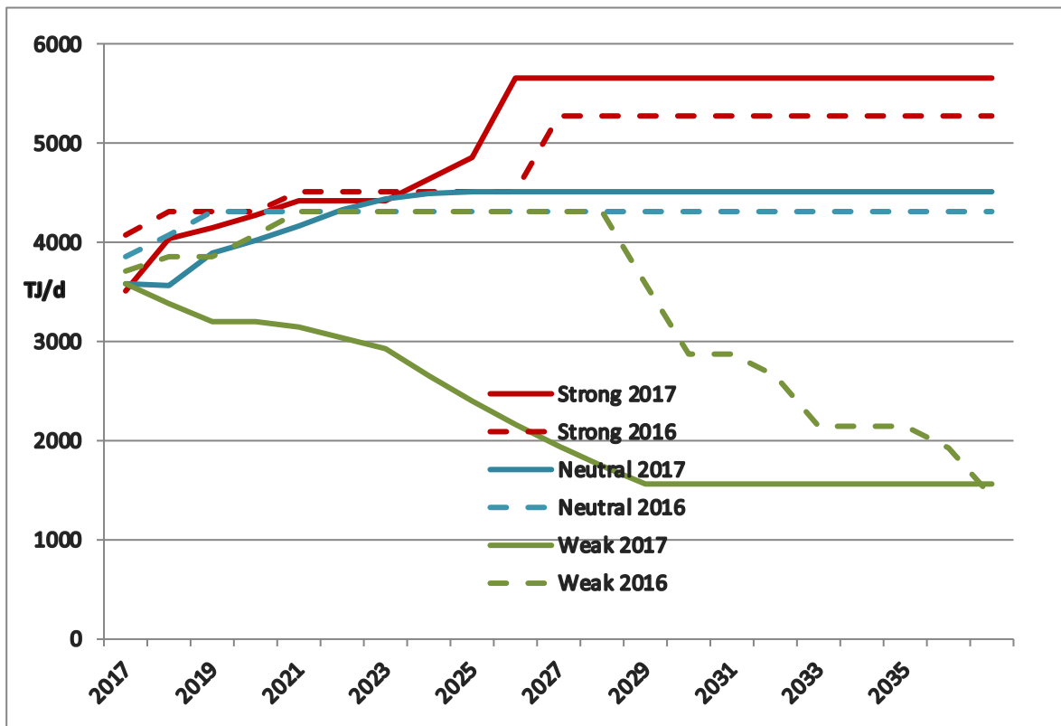
Figure 4-7 Peak winter gas demand
