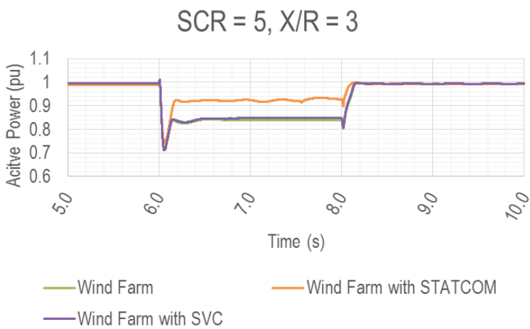
Figure 35 Active power
