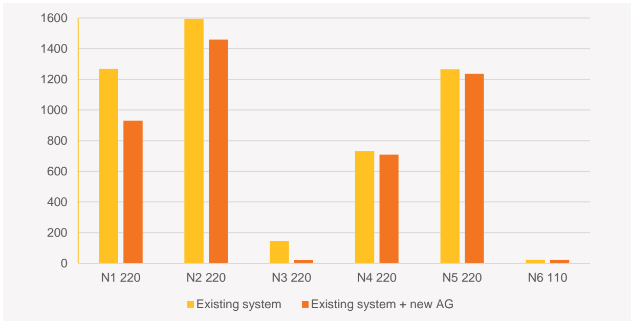
Figure 5 Assessment of available fault level at six Tasmanian busbar locations (new AG at N1 220)
