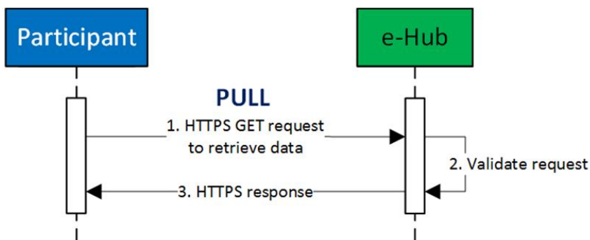
Figure 2 PULL mechanism
