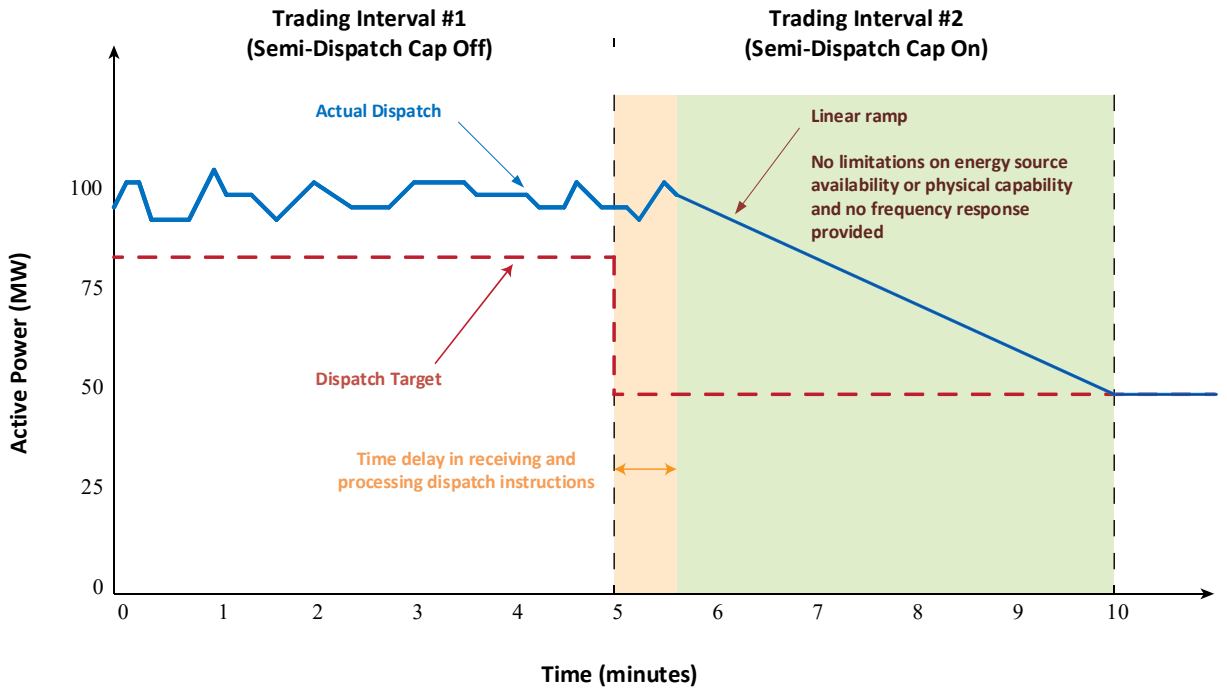
Figure 6 Semi-scheduled generating unit linear ramping with no limiting factors
